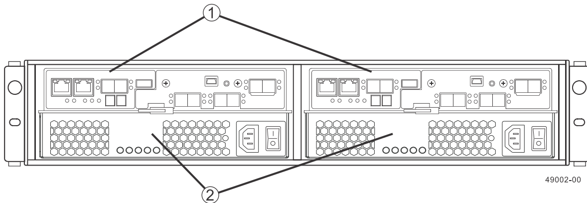
Figure 1. Power-Fan Canister and Controller Canister
